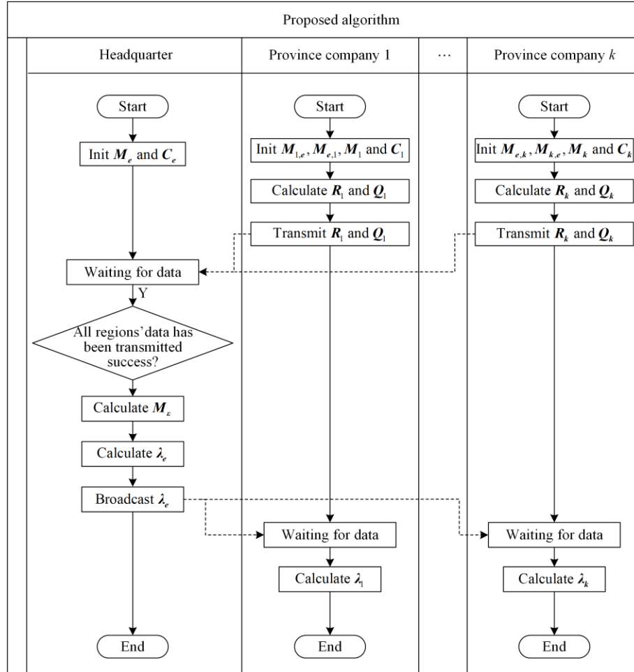
Fig. 5. Flow chart for the proposed method.
