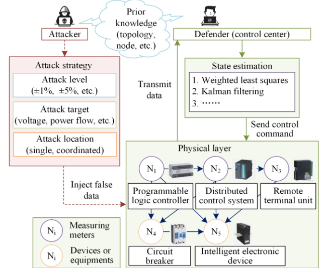
Fig. 1. Overall architecture of the proposed system model under the FDI attacks in the context of CPPS.
