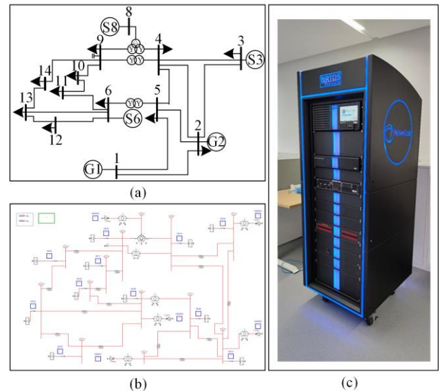
Fig. 9. IEEE 14-bus system and RTDS model. (a) IEEE 14-bus system. (b) System model construction. (c) NovaCor hardware platform of RTDS.
