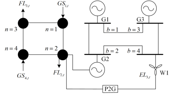
Fig. 4. Topology of the 4-node-4-bus IEGS.
