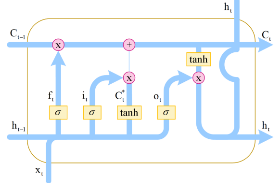
Fig. 5. LSTM structure.
