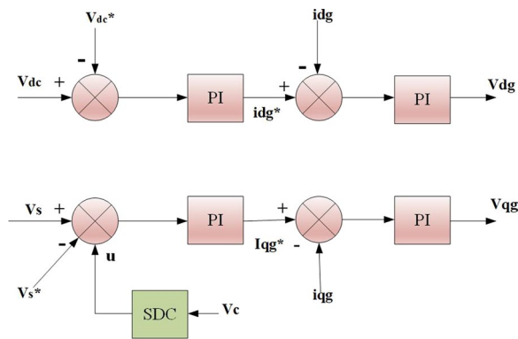
Fig. 6 With an auxiliary SSR damping at q-axis loop
