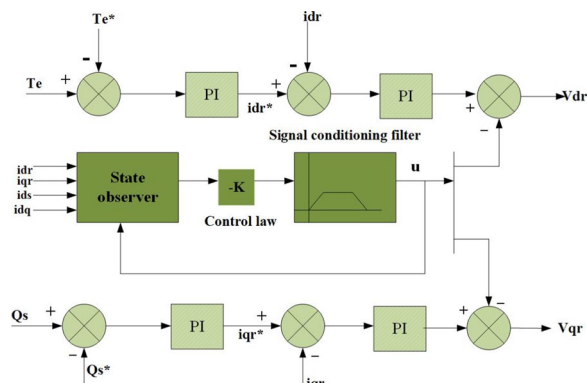
Fig. 11 The supplementary SSI damping Observer-based state-feedback controller
